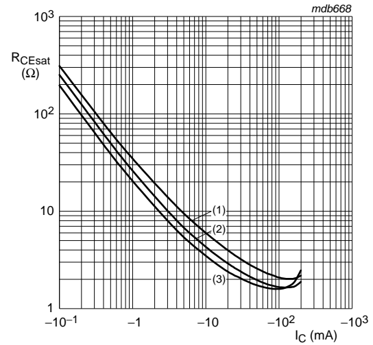
I_C/I_B = 10 (1) T_{amb} = 150\text{ °C} (2) T_{amb} = 25\text{ °C} (3) T_{amb} = -55\text{ °C}
