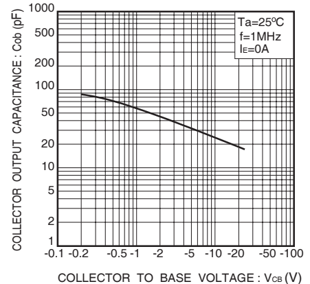
Fig.6 Collector output capacitance vs. collector-base voltage
