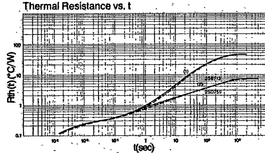
Thermal Resistance vs. t
