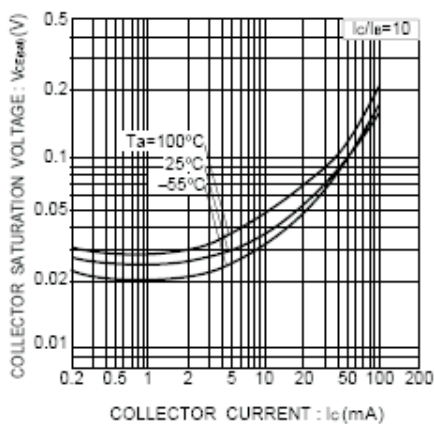
Fig.7 Collector Emitter Saturation Voltage vs. Collector Current
