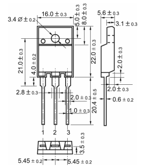
TO-3PML
