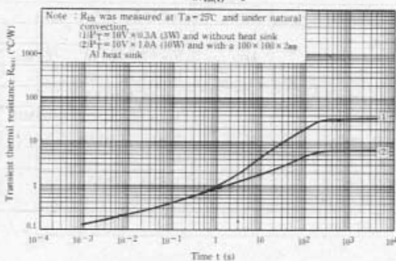
R_{th(t)} - t
