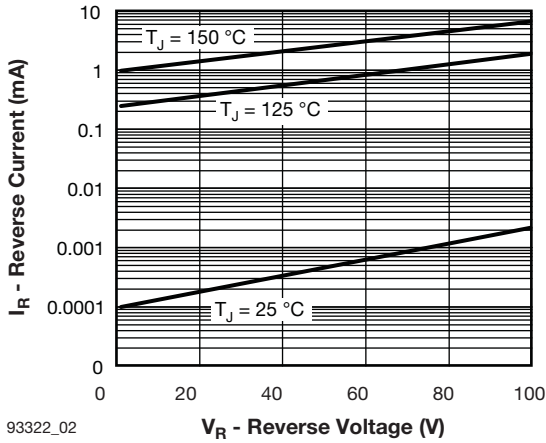
93322_02 Fig. 2 - Typical Values of Reverse Current vs. Reverse Voltage
