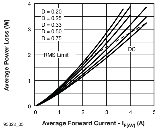
93322_05 Fig. 5 - Forward Power Loss Characteristics
