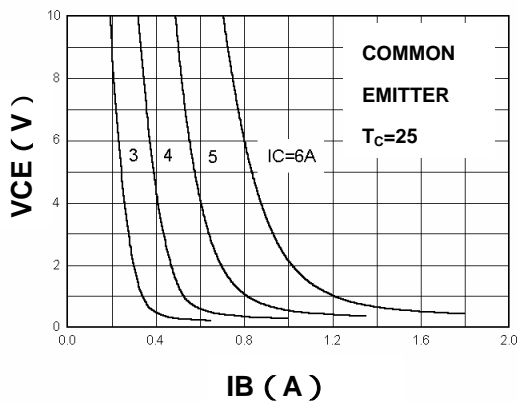
VCE - IB
