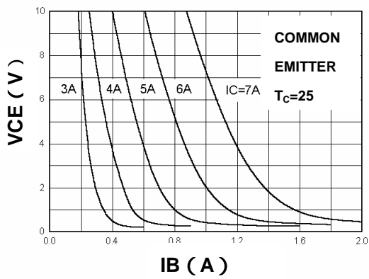
VCE - IB
