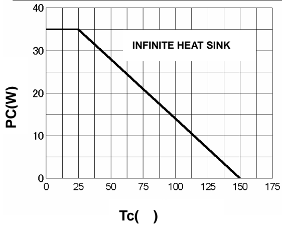
PC-TC
