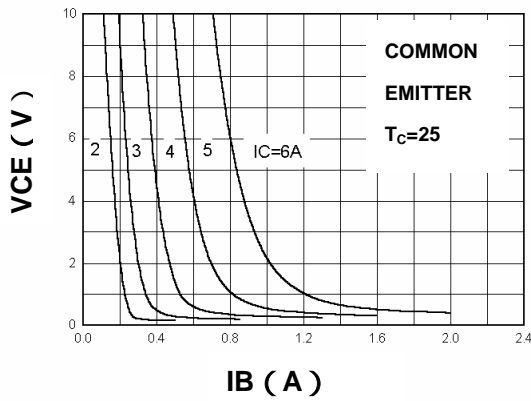
VCE - IB
