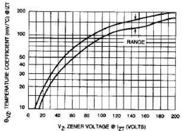
Fig. 6-UNITS 10 TO 200 VOLTS
