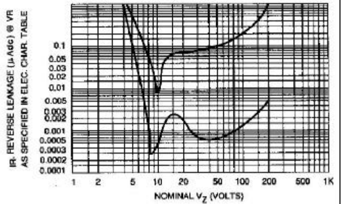
Fig. 4-TYPICAL REVERSE LEAKAGE
