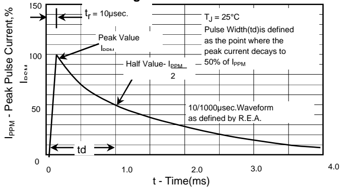
Fig.3 - Pulse Waveform
