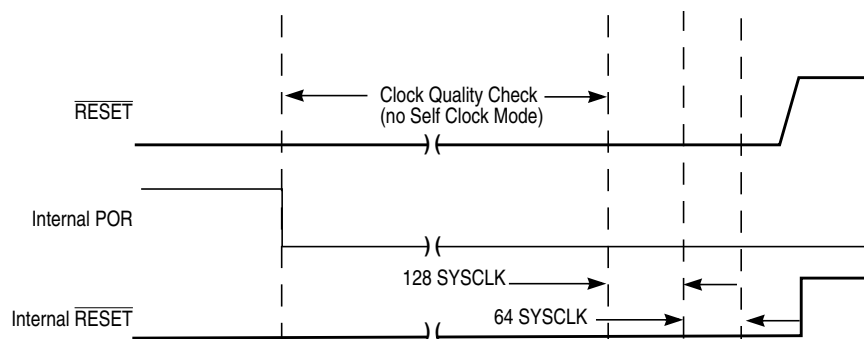
Figure 2-27. \overline{\text{RESET}} Pin Held Low Externally
