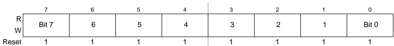
Figure 8-16. PWM Channel Duty Registers (PWMDTY x )
