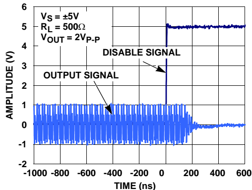
FIGURE 26. DISABLE TIME
