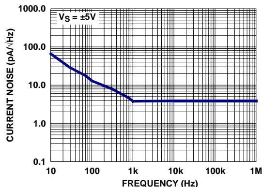
FIGURE 28. EQUIVALENT INPUT CURRENT NOISE vs FREQUENCY
