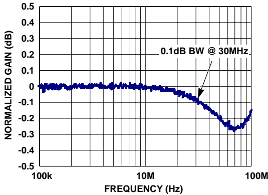
FIGURE 3. 0.1dB BANDWIDTH
