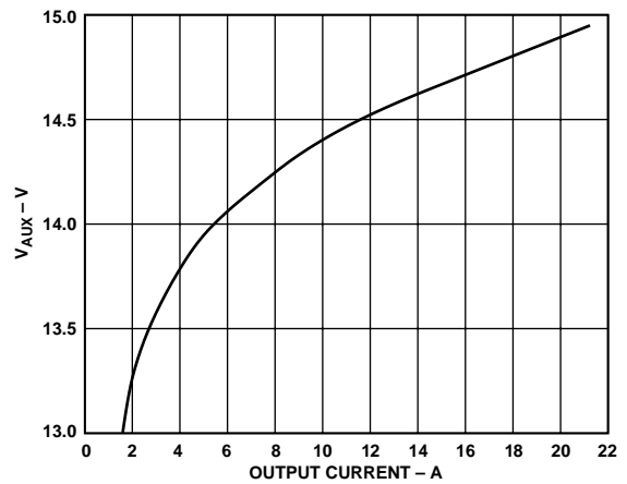
Figure 29. V_{AUX} vs. Converter Output Current (ADDC02805SA)
