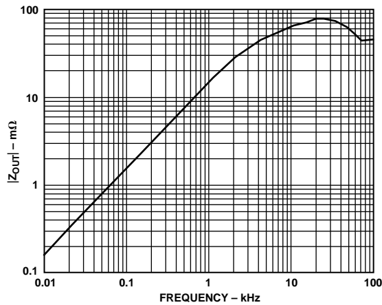
Figure 15. Incremental Output Impedance (Magnitude) (ADDC02805SA)
