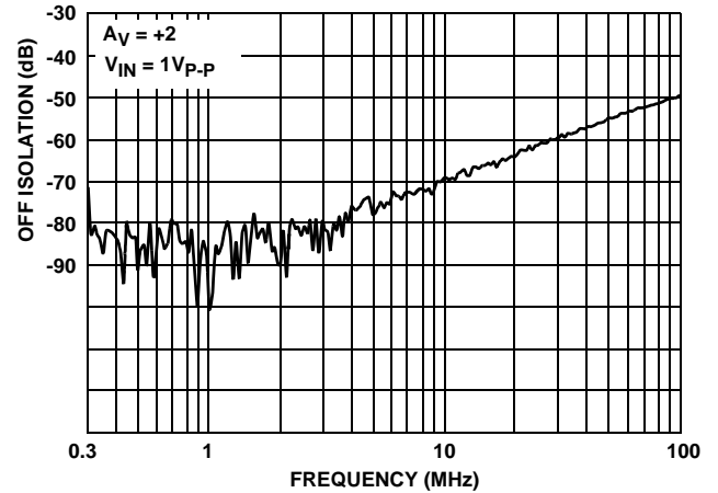
FIGURE 20. OFF ISOLATION
