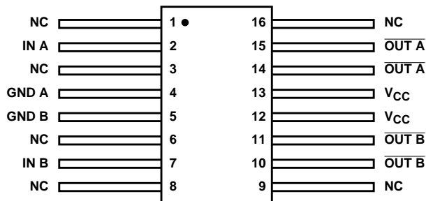
HS-4423RH, HS-4423BRH (FLATPACK CDFP4-F16) TOP VIEW
