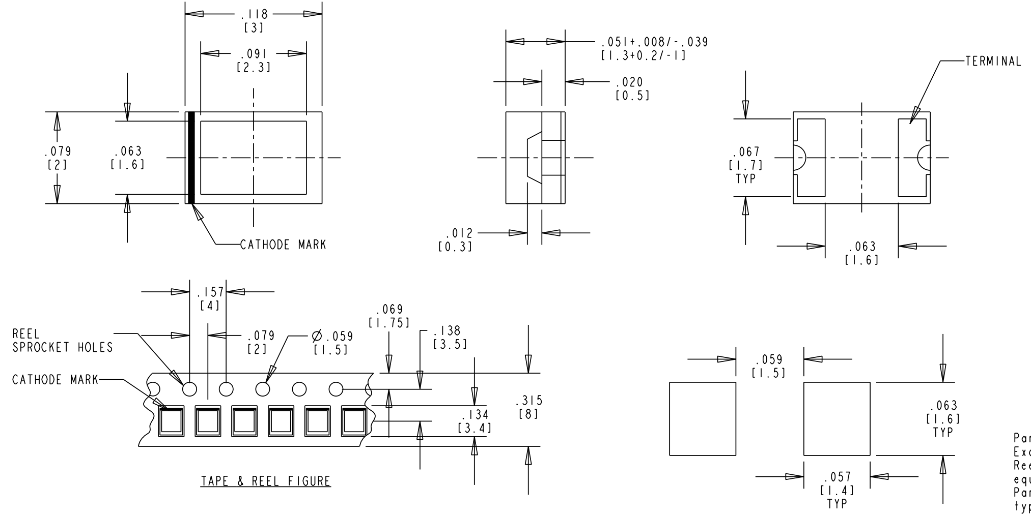
SOLDER PAD LAYOUT
