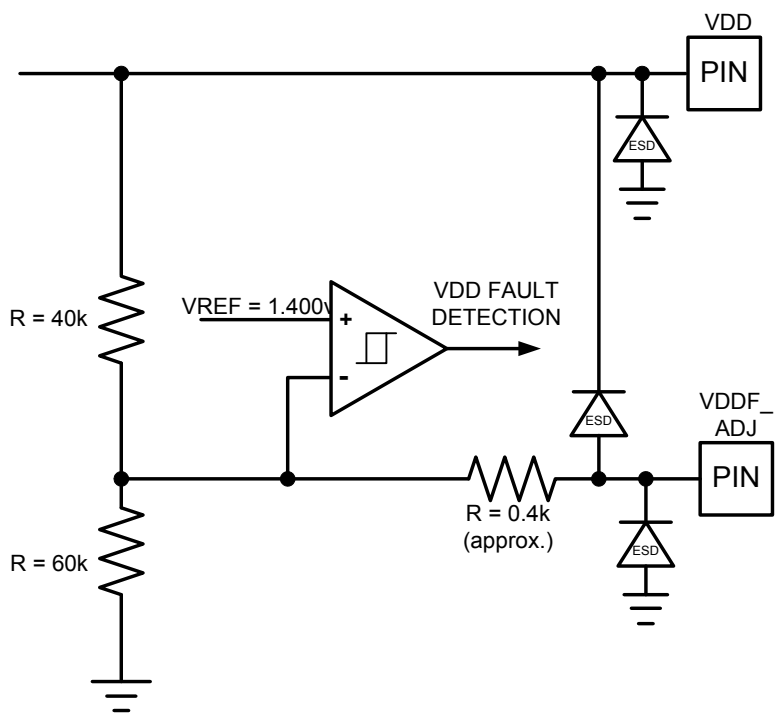
Figure 18: VDDF_ADJ
