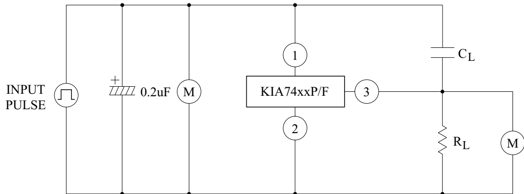
TEST CIRCUIT 2.
