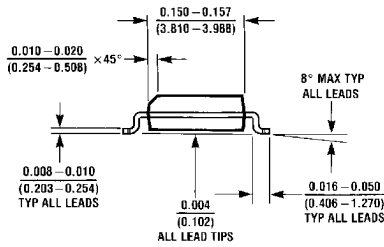
14-Lead Small Outline Integrated Circuit—JEDEC SOIC (M) Package Number M14A
