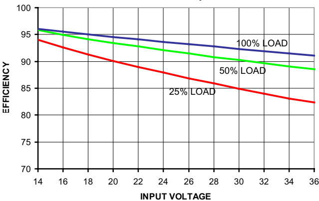
7812SR Efficiency
