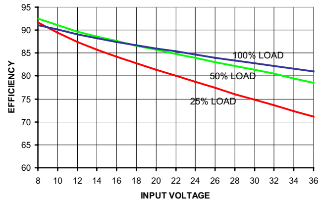
7805SR Efficiency
