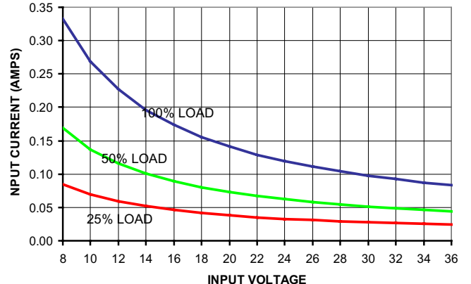
7805SR Input Current
