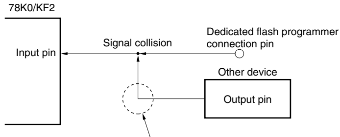
Figure 27-9. Signal Collision (Input Pin of Serial Interface)
