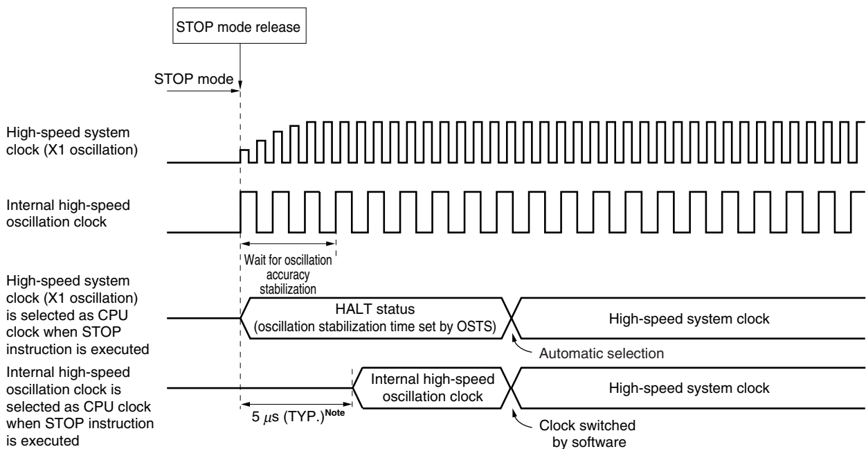
Figure 22-5. Operation Timing When STOP Mode Is Released
