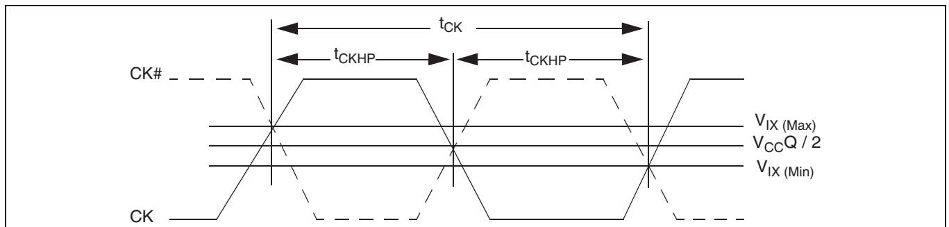
Figure 28 Clock characteristics
