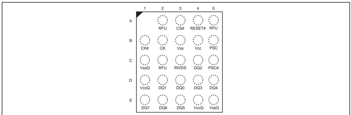
Figure 37 24-ball FBGA, 5 × 5 ball footprint, top view
