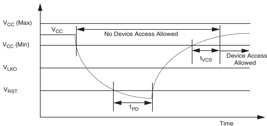
Figure 21 Power down or voltage drop
