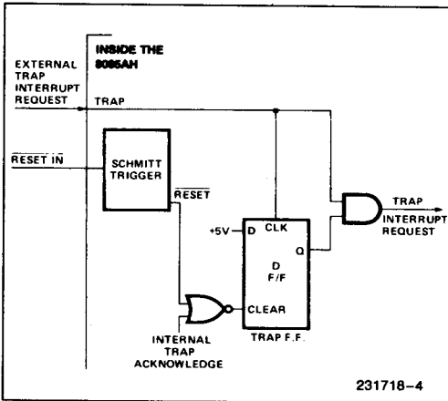
Figure 4. TRAP and RESET In Circuit
