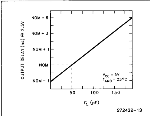
Figure 13. Typical Output Delay Variations Versus Load Capacitance
