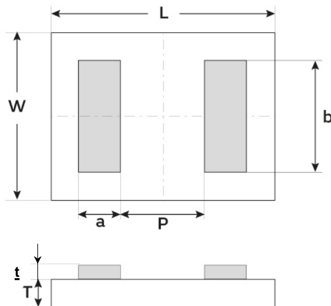
Figure 6 – Layout view
