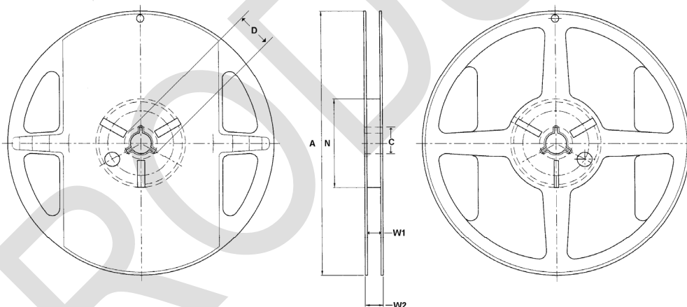
Figure 7 - Reel drawing
