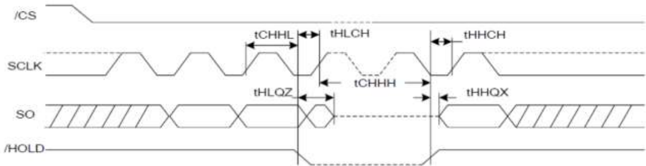
Figure 5. Hold Timing
