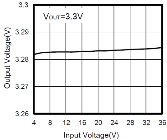
9. Line Regulation
