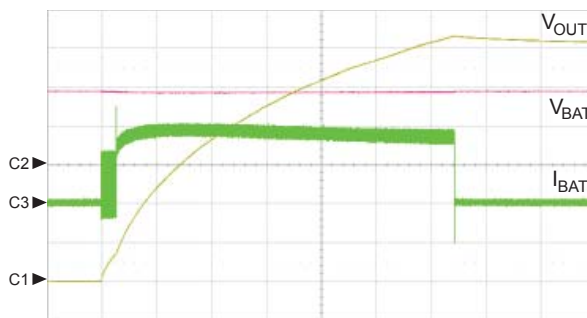
Figure 11. Input current waveforms with Li+ battery connected through 4.7 \mu H inductor and 4.7 \mu F capacitor, C_{OUT} = 100 \mu F, V_{IN} = V_{BAT} = 3.6 V, Ch1: V_{OUT} = 50 V/div, Ch2: V_{BAT} = 2 V/div, Ch3: I_{BAT} = 200 mA/div, t = 1 s/div
