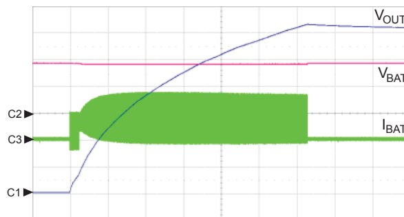
Figure 10. Input current waveforms with Li+ battery connected by 5-in. wire and decoupled by 4.7 \mu F capacitor, C_{OUT} = 100 \mu F, V_{IN} = V_{BAT} = 3.6 V, Ch1: V_{OUT} = 50 V/div, Ch2: V_{BAT} = 2 V/div, Ch3: I_{BAT} = 500 mA/div, t = 1 s/div
