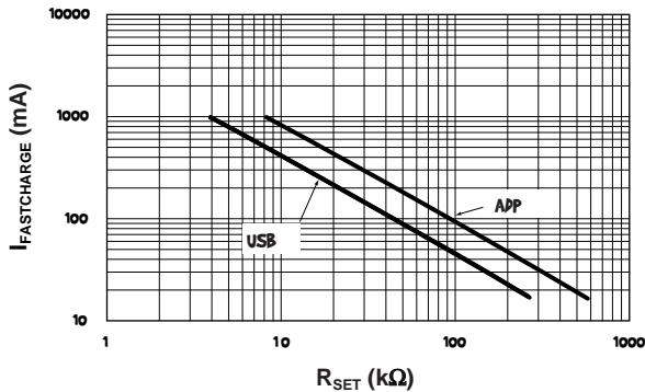
Figure 2: I FASTCHARGE VS. R SET .
