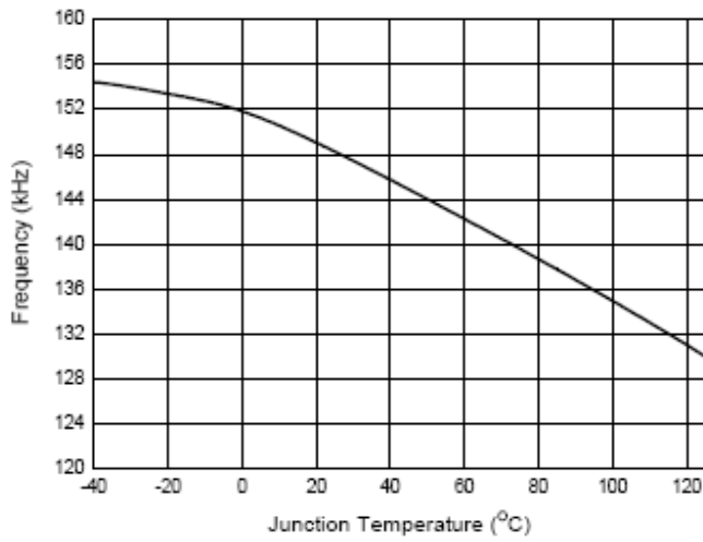
Figure 15. Switching Frequency vs. Junction Temperature
