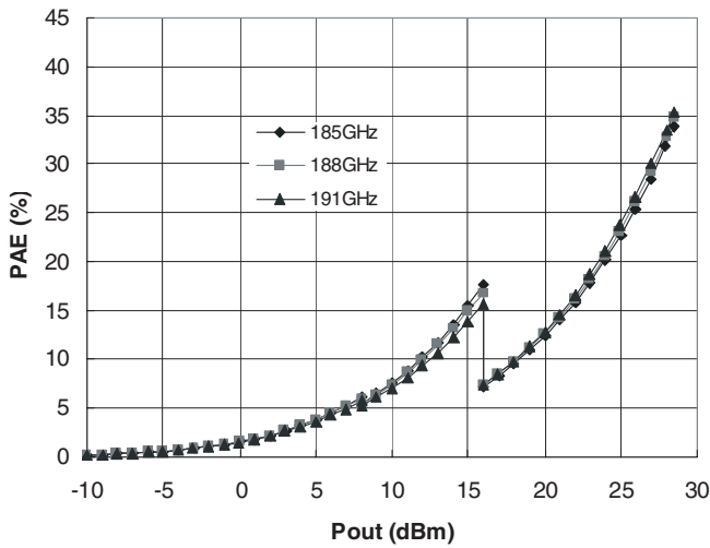
Figure 3. Power Added Efficiency vs. Output Power
