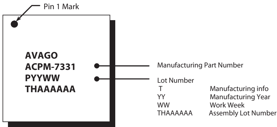
Figure 13. Marking Specifications
