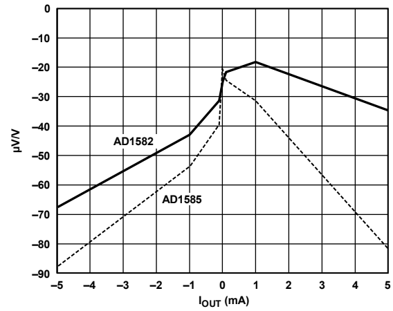
Figure 7. Line Regulation vs. I_{OUT}
