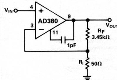
Figure 30. Video Amplifier
