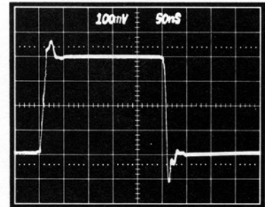
Figure 26c. Unity Gain Small Signal Response
