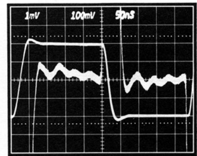
Figure 25c. Unity Gain Inverter Small Signal Response
