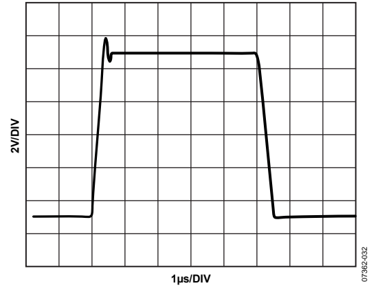
Figure 27. Large-Signal Pulse Response, Gain = 1/2
