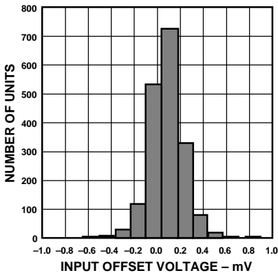
Figure 4. Typical Distribution of Input Offset Voltage (1855 Units)
