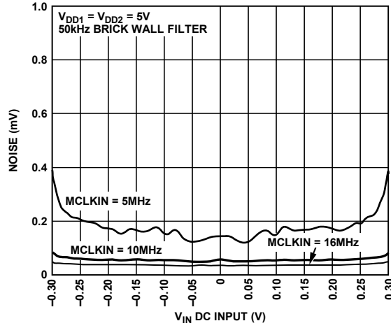
Figure 20. RMS Noise Voltage vs. V_{IN} DC Input
