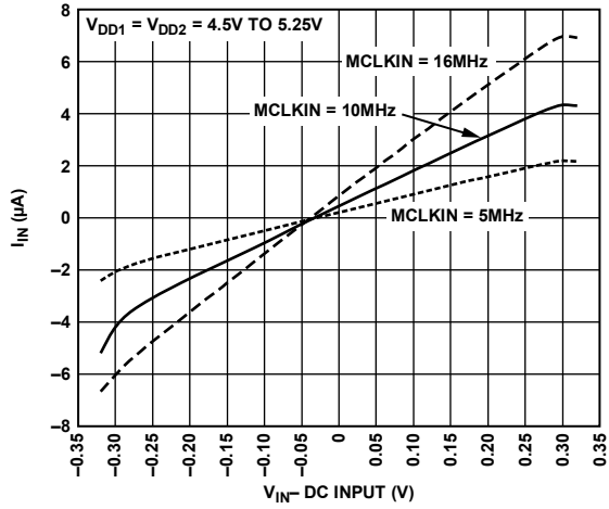
Figure 18. I_{IN} vs. V_{IN} —DC Input
