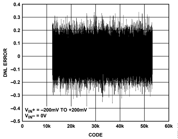
Figure 10. Typical DNL (±200 mV Range)
