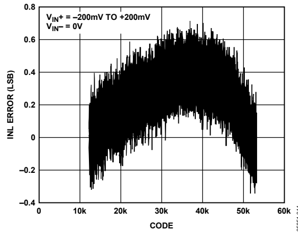
Figure 11. Typical INL (±200 mV Range)
