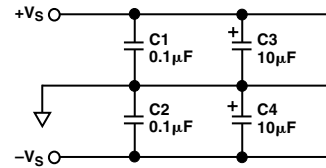
Supply Bypassing
