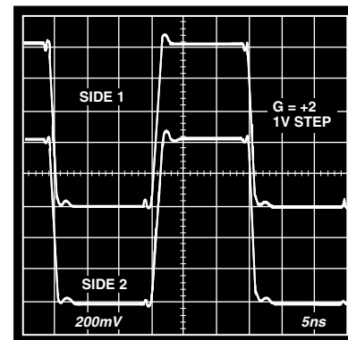
Figure 2. 1 V Step Response, G = +1
