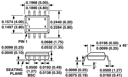
8-Lead Plastic SOIC (SO-8)
