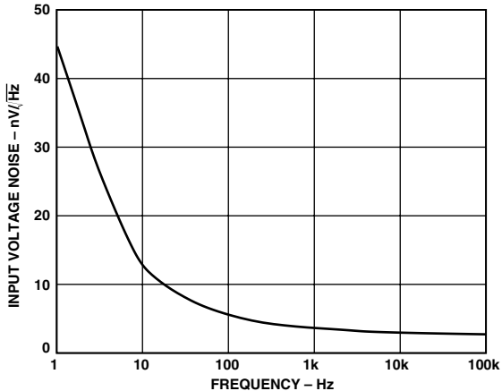
Figure 17. Noise vs. Frequency; V_S = \pm 5\text{ V}
