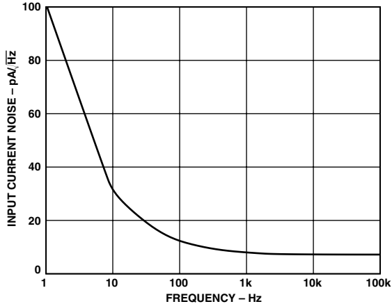
Figure 18. Noise vs. Frequency; V_S = \pm 5\text{ V}
