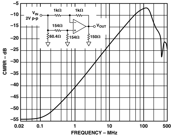
Figure 20. CMRR vs. Frequency; V_S = \pm 5\text{ V}
