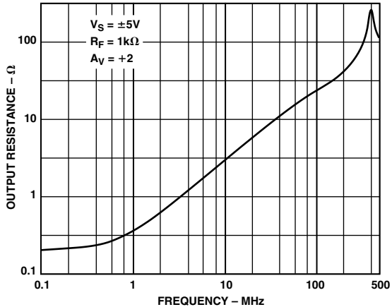
Figure 16. Output Resistance vs. Frequency; V_S = \pm 5\text{ V}
