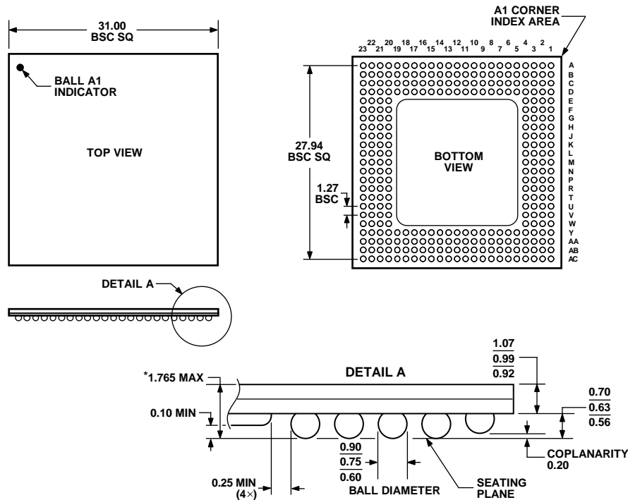
*COMPLIANT TO JEDEC STANDARDS MO-192-BAN-2 WITH THE EXCEPTION TO PACKAGE HEIGHT. Figure 73. 304-Ball Ball Grid Array, Thermally Enhanced [BGA_ED] (BP-304) Dimensions shown in millimeters
