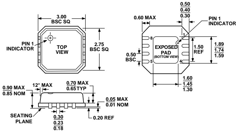
Figure 71. 8-Lead Lead Frame Chip Scale Package [LFCSF_VD]
