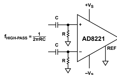
CAPACITOR COUPLED
