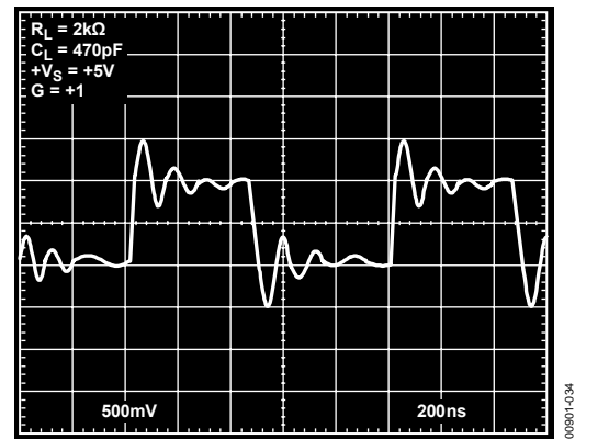
Figure 34. Pulse Response, +V_S = +5\text{ V} , G = +1 , C_L = 470\text{ pF}
