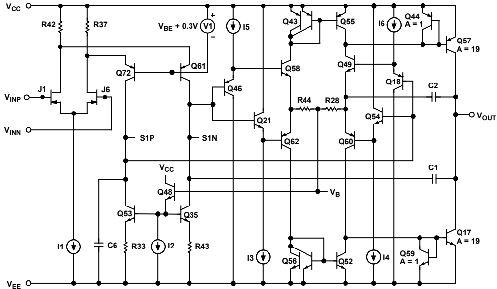
Figure 36. Simplified Schematic
