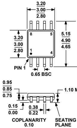
Figure 45. 8-Lead Mini Small Outline Package [MSOP] (RM-8) Dimensions shown in millimeters
