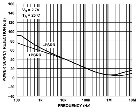
Figure 10. Power Supply Rejection vs. Frequency
