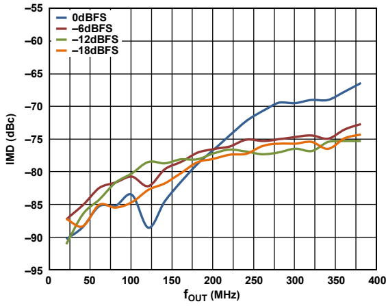
Figure 11. IMD vs. f_{OUT} over Digital Scale, 4x Interpolation, f_{DATA} = 400\text{ MSPS} , I_{FS} = 20\text{ mA}
