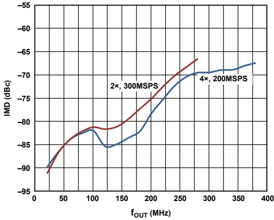
Figure 10. IMD vs. f_{OUT} over f_{DATA} and Interpolation, Digital Scale = 0 dBFS, I_{FS} = 20\text{ mA}
