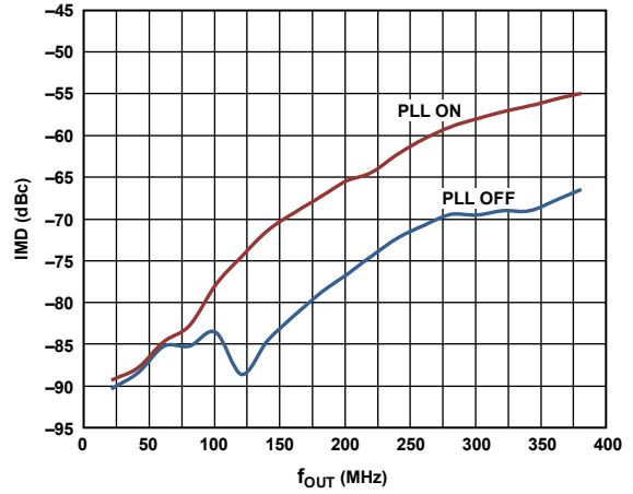
Figure 13. IMD vs. f_{OUT} , 4x Interpolation, f_{DATA} = 200\text{ MSPS} , Digital Scale = 0 dBFS, I_{FS} = 20\text{ mA} , PLL On and PLL Off
