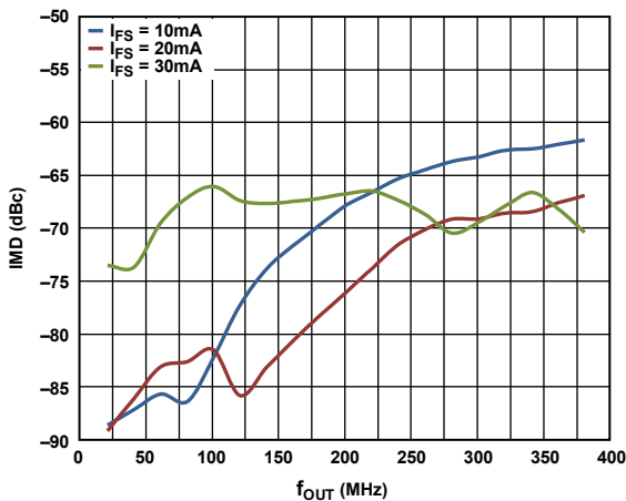
Figure 12. IMD vs. f_{OUT} over Full-Scale Current, 4x Interpolation, f_{DATA} = 400\text{ MSPS} , Digital Scale = 0 dBFS
