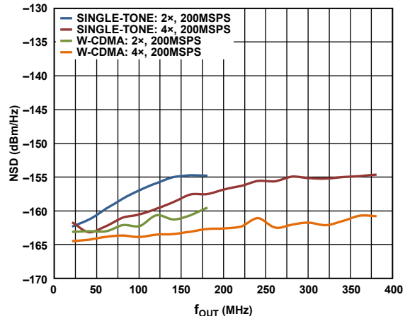
Figure 14. NSD vs. f_{OUT} over Interpolation, Single-Tone and W-CDMA Signals, f_{DATA} = 200\text{ MSPS} , Digital Scale = 0 dBFS, I_{FS} = 20\text{ mA} , PLL Off
