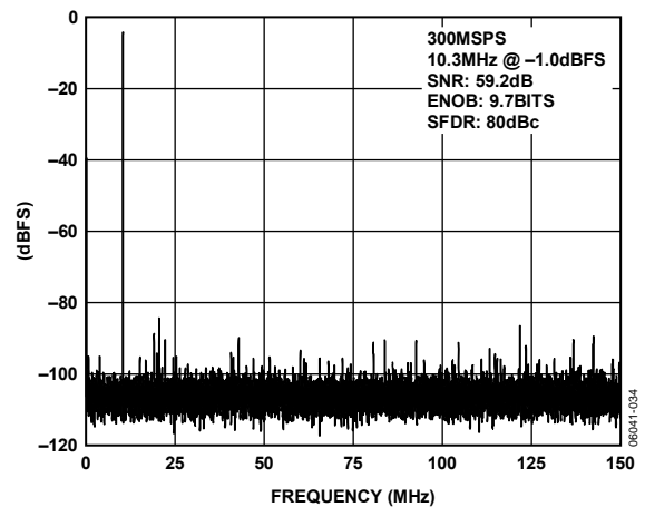
Figure 20. AD9211-300 64k Point Single-Tone FFT; 300 MSPS, 10.3 MHz
