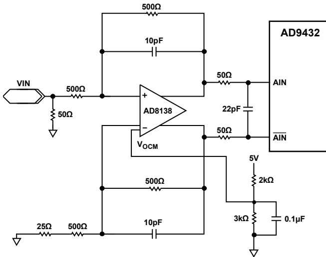
Figure 29. AD8138/AD9432 Schematic
