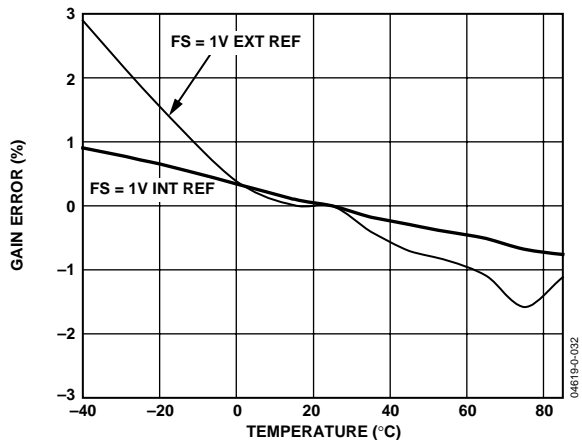
Figure 32. Full-Scale Gain Error vs. Temperature, A_{IN} = 70.3 \text{ MHz @ } -0.5 \text{ dBFS, } 250 \text{ MSPS, } FS=1
