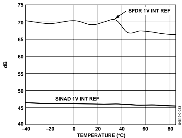
Figure 33. SINAD, SFDR vs. Temperature, A_{IN} = 70 \text{ MHz @ } -1 \text{ dBFS, } 250 \text{ MSPS}
